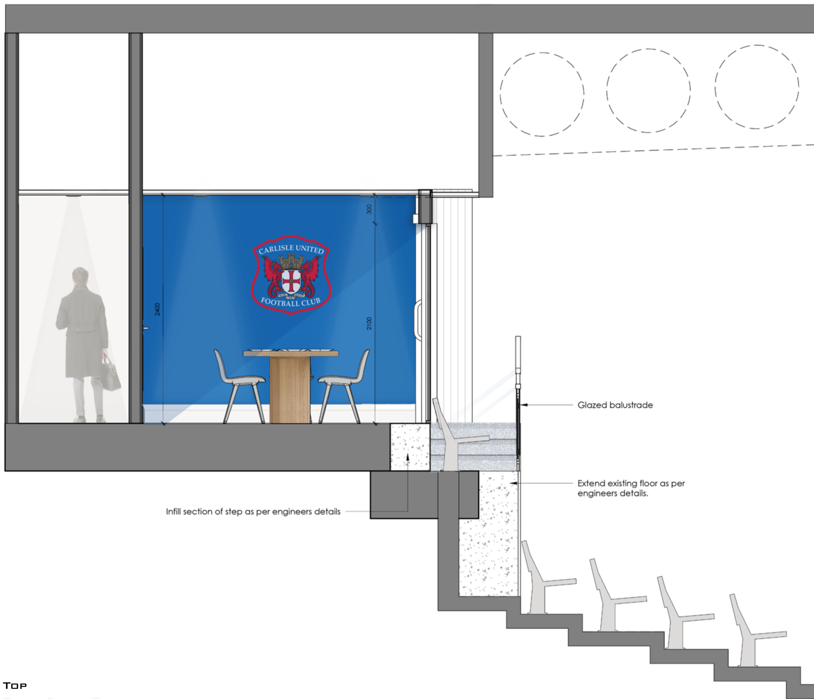
TOP LEFT EXECUTIVE BOX SECTION, SCALE 1:50
